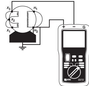
b. Low voltage winding to high voltage winding and ground
