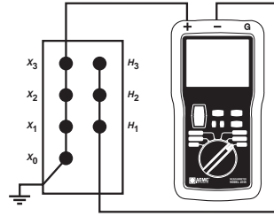
a. High voltage winding to low voltage winding and ground
