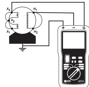
d. High voltage winding to ground
