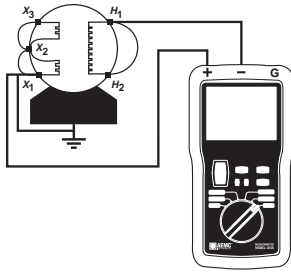
a. High voltage winding to low voltage winding and ground
