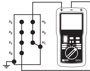
c. High voltage winding to low voltage winding
