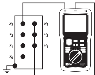
e. High voltage winding to low voltage winding
